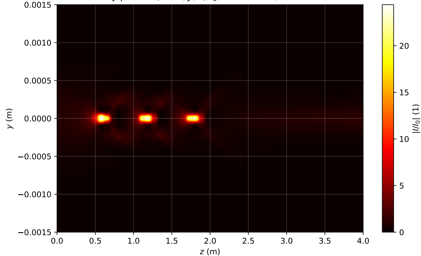
Intensity profile I(x=0, y, z)/I_0 , P_{in}=4.5P_{cr} , artificial time
